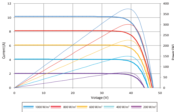
Current-Voltage & Power-Voltage Curve (375S)
